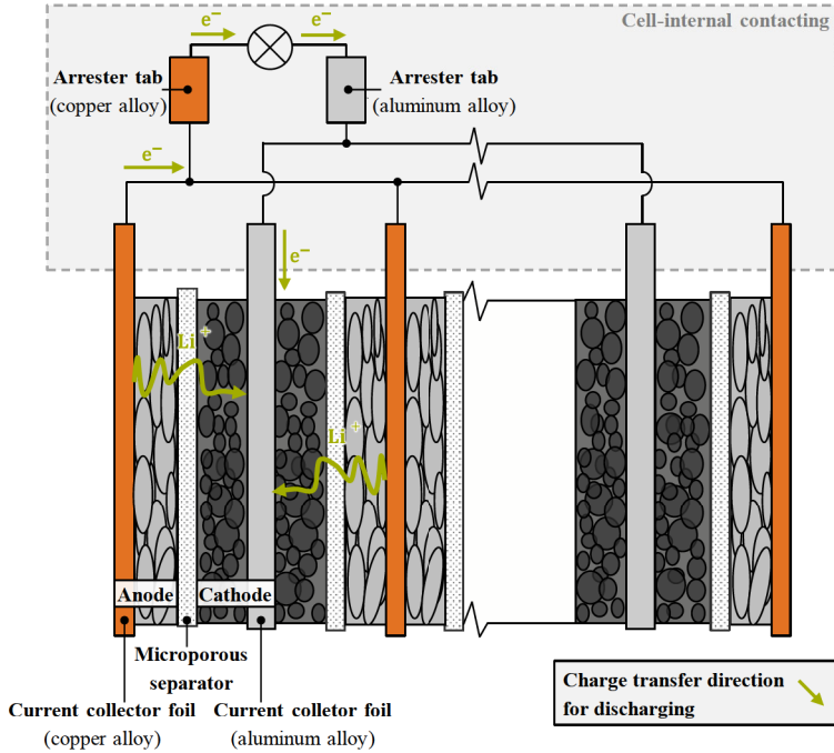
Figure 1: Cell stack of a multi-layer LIB cell during discharge with a focus on the cell-internal contacting, i.e., the electrical connection of the individual anode and cathode layers; the dimensions are not to scale.
