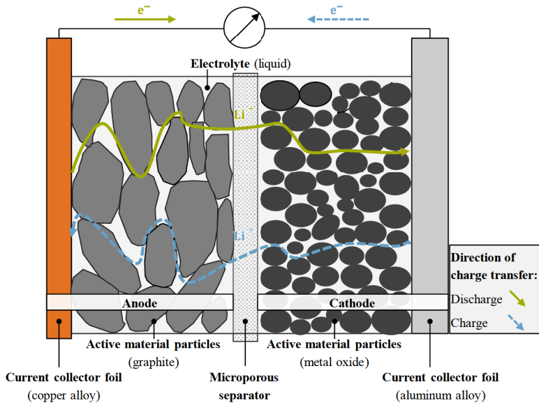
Figure 2: Schematic drawing of a lithium-ion elementary cell; adapted from VUORILEHTO (2013, p. 22); the dimensions are not to scale.
